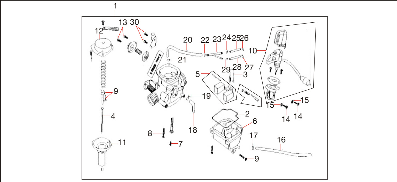
FIG - 3: CARBURETOR
