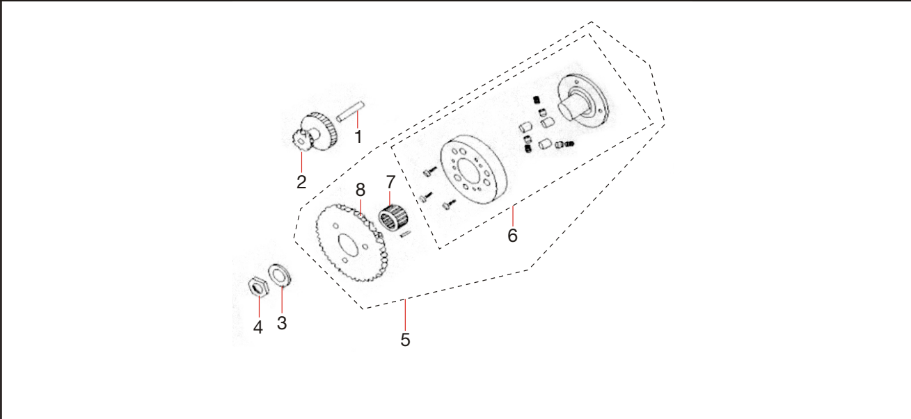
FIG - 17: STARTER CLUTCH
