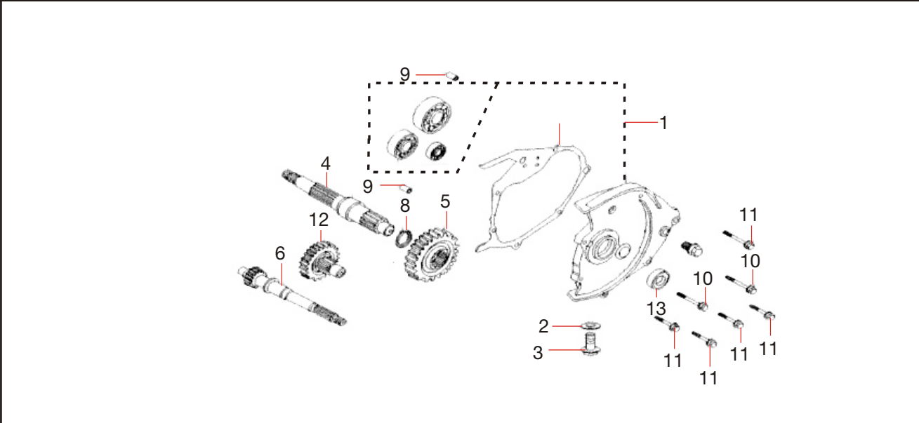
FIG - 19: TRANSMISSION
