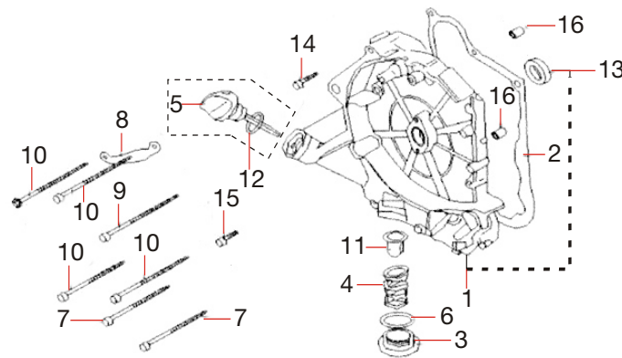
FIG - 16: RIGHT CRANKCASE COVER
