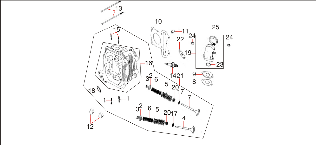
FIG - 8: CYLINDER HEAD
