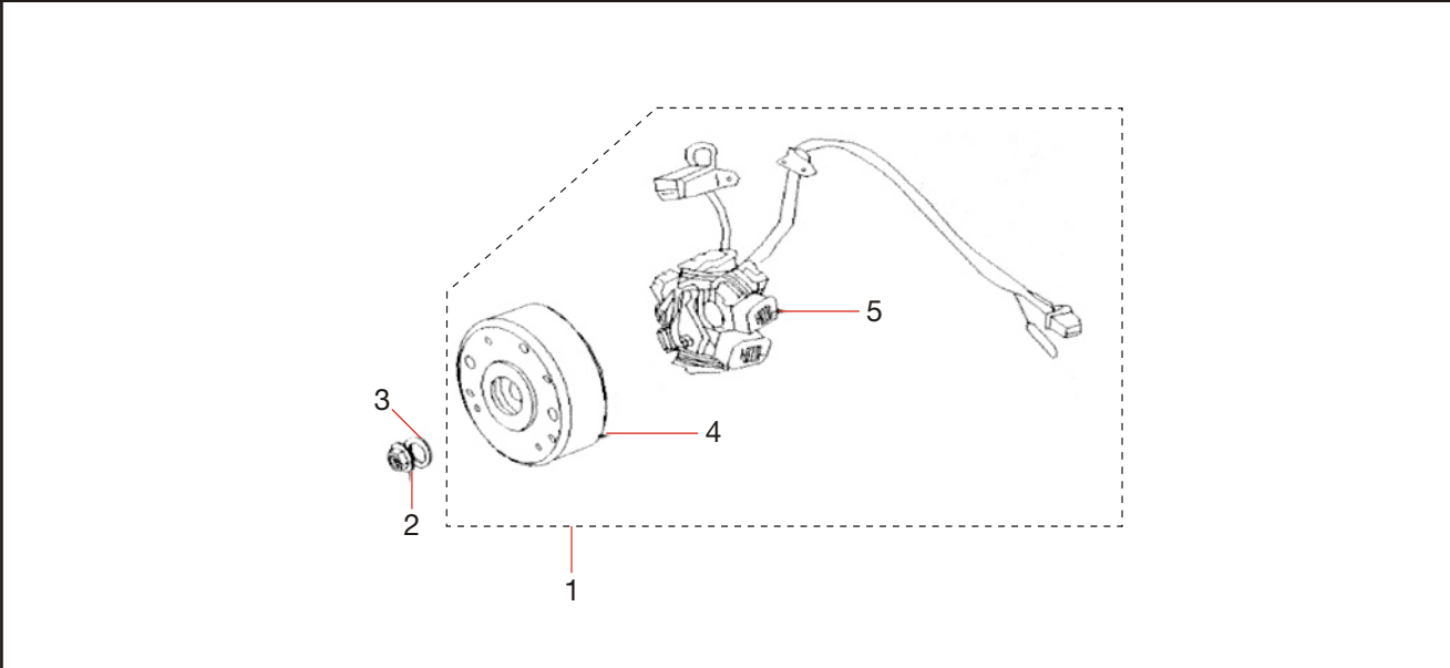
FIG - 14: MAGNETO
