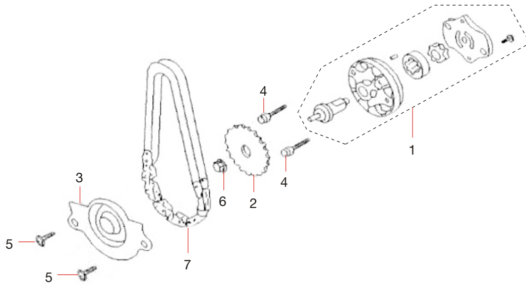
FIG - 15: OIL PUMP
