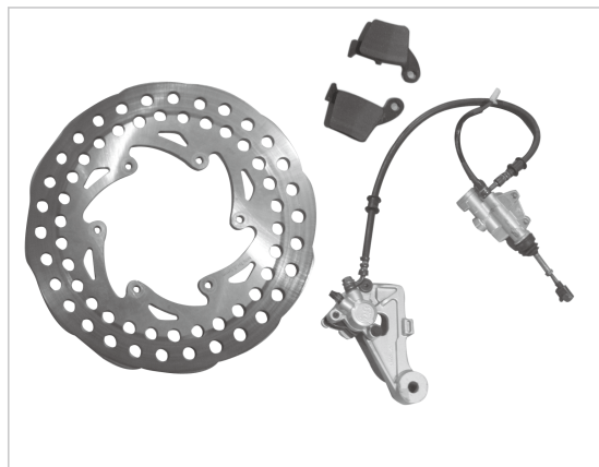
Structure drawing of disc brake
