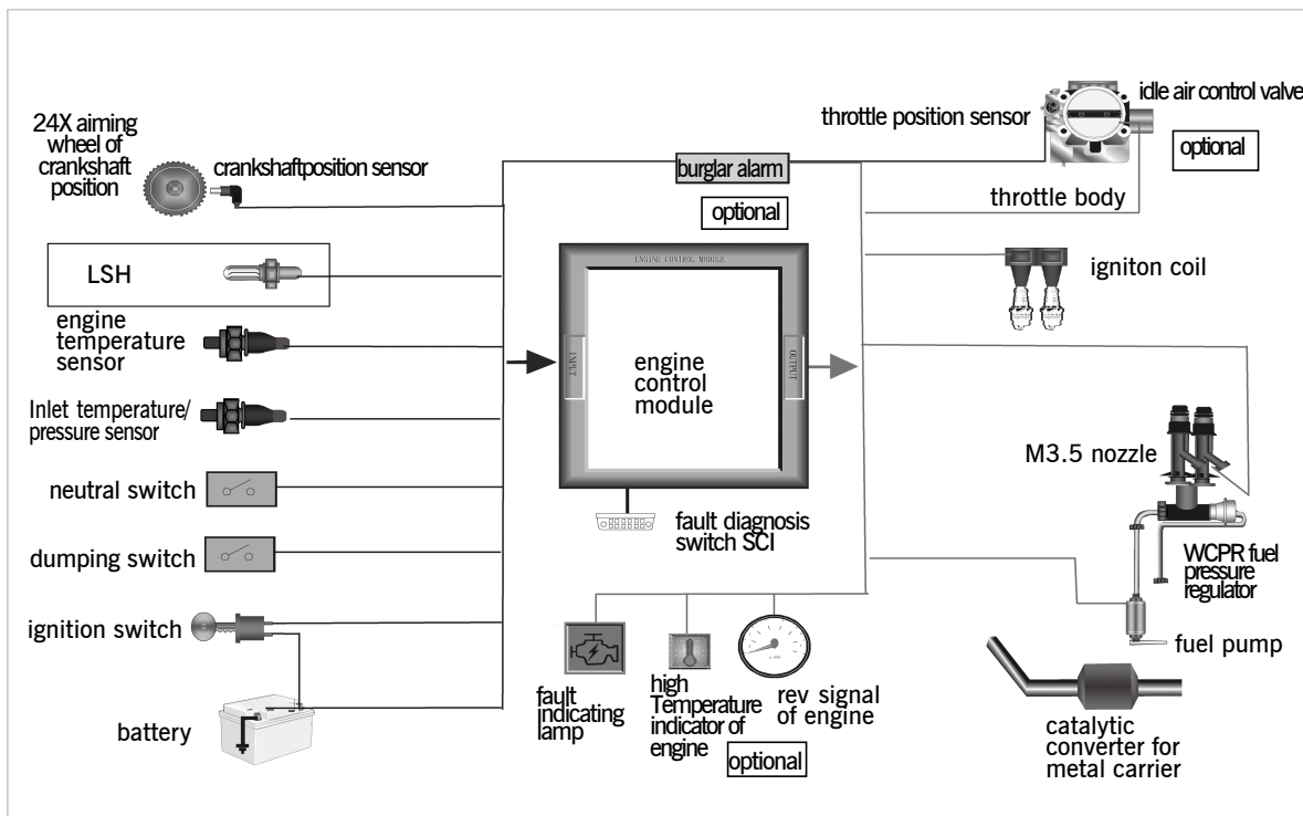
Structural drawing of EFI system
